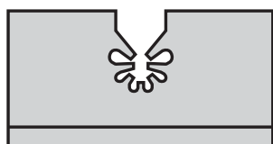
CN-12133 L= 38 mm H= 20 mm Endoscope holder, double one side 12 mm open one side from \varnothing 3 to \varnothing 8 mm
