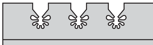
CN-12132 L= 72 mm H= 30 mm Instruments holder from \varnothing 3 to \varnothing 8 mm
