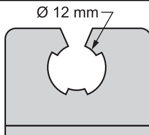
CN-12139 L= 38 mm H= 29 mm Endoscope holder, \varnothing 12 mm closed
