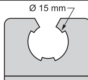
CN-12140 L= 38 mm H= 29 mm Endoscope holder, \varnothing 15 mm closed
