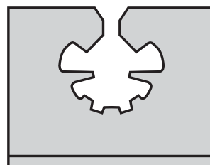
CN-12134 L= 38 mm H= 30 mm Endoscope holder, double one side 12 mm open one side from \varnothing 3 to \varnothing 8 mm
