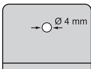
CN-12135 L= 38 mm H= 29 mm Endoscope holder, \varnothing 4 mm closed
