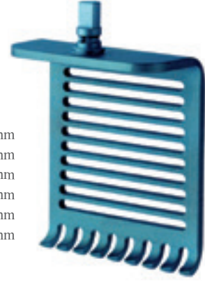
BM-2231 60 x 35 mm BM-2232 60 x 40 mm BM-2233 60 x 45 mm BM-2234 60 x 55 mm BM-2235 60 x 65 mm BM-2236 60 x 75 mm BM-2237 60 x 85 mm Titanyum bleydler Blades titanium
