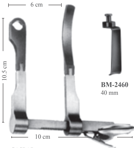
CASPAR BM-2440 Komple/Complete BM-2441 - BM-2442 - BM-2450
