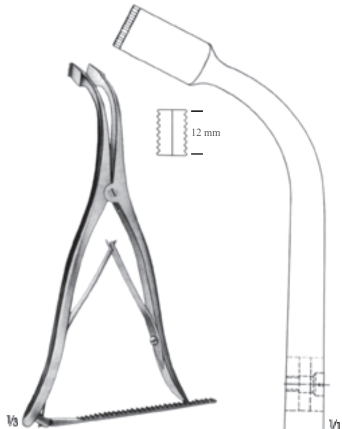
INGE BM-2550 27.5 cm
