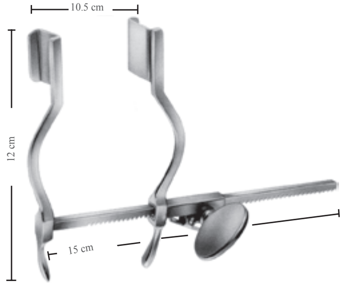
HERTZLER BM-2675 Bleyd/Blades 20 x 25 mm
