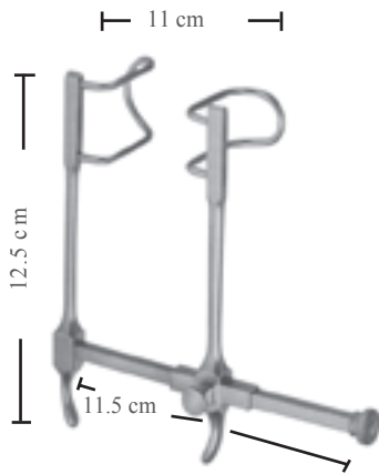
GOSSET BM-2670 Bleyd/Blades 38 mm
