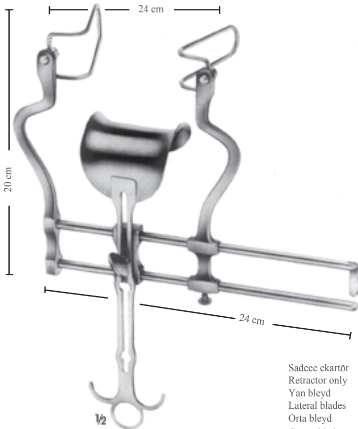
BALFOUR BM-2735 - BM-2738 Komple/Complete
