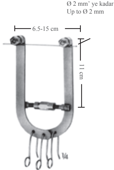
BT-1802 Ayarlı küçük boy, üç kancalı traksiyon aleti Wire traction bow, adjustable, with 3 hooks, small size BT-1935 Uygun anahtar BT-1935 Suitable wrench
