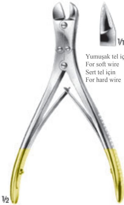
REILL BR-8275 Kemiğe yakın olan telleri kesme For cutting off wires close to the bone 17.5 cm
