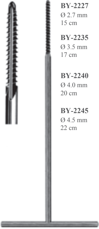
BY-2227 - BY-2245 Kemik tapları/Bone taps
