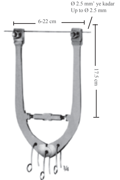
BT-1801 Ayarlı büyük boy, üç kancalı traksiyon aleti Wire traction bow, adjustable, with 3 hooks, large size BT-1935 Uygun anahtar BT-1935 Suitable wrench
