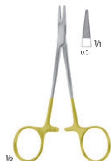
CONVERSE BF-5130 13 cm
