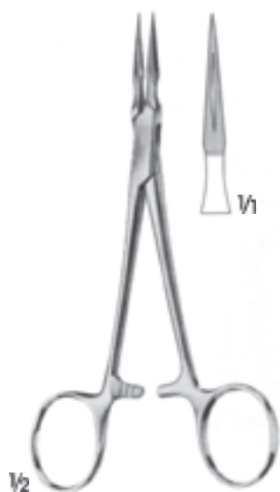
STIEGLITZ BD-6110 Kıymık penset Splinter forceps 14 cm
